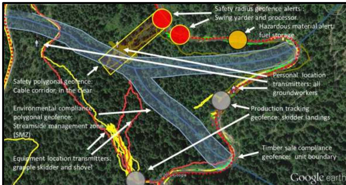
Figure 1: Example of a digitally defined harvest unit, coupling various geofence applications with real-time positional transmitters on all equipment and ground workers
